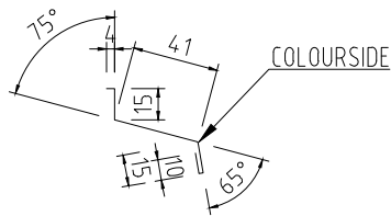
UNDERBLECK FÄNSTER 40 Tj=0,6 L=1200, 1500, 2000mm KB=85mm
